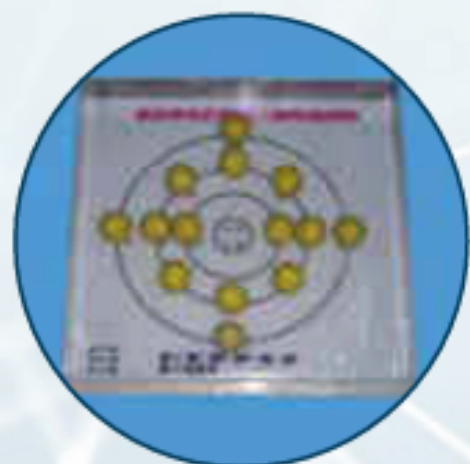
SILICON ELECTRONIC CONFIGURATION
