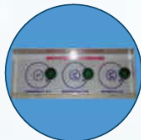
ISOTOPES OF HYDROZEN
